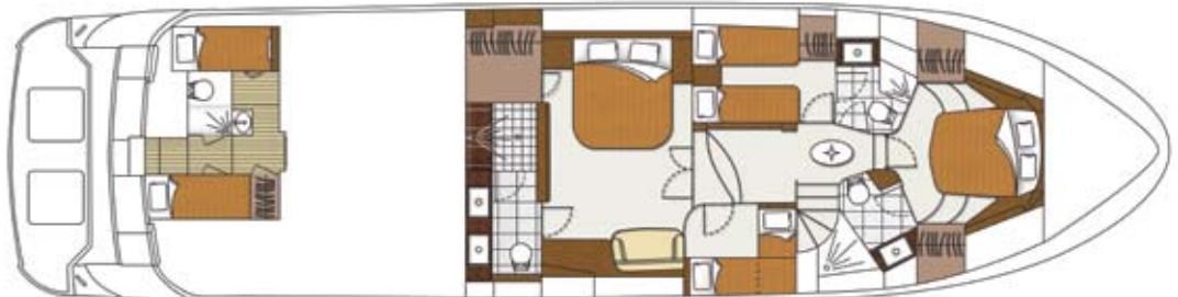
Accommodations Deck Shown with optional Fourth Stateroom & Double Crew Quarters
